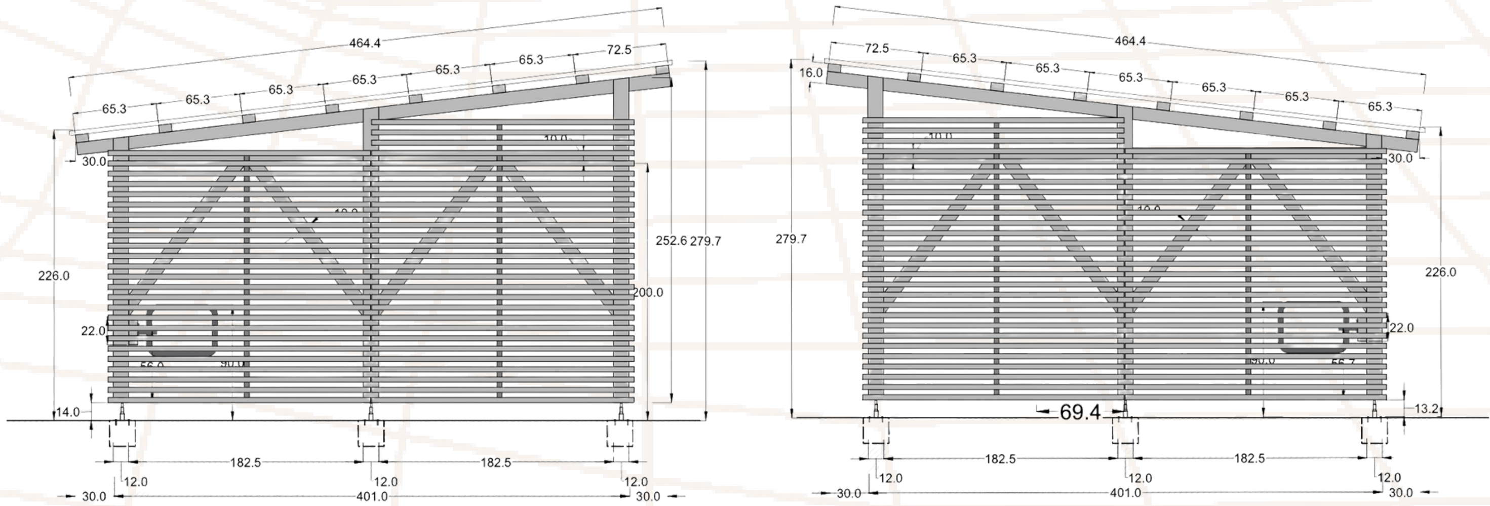
Façade A
